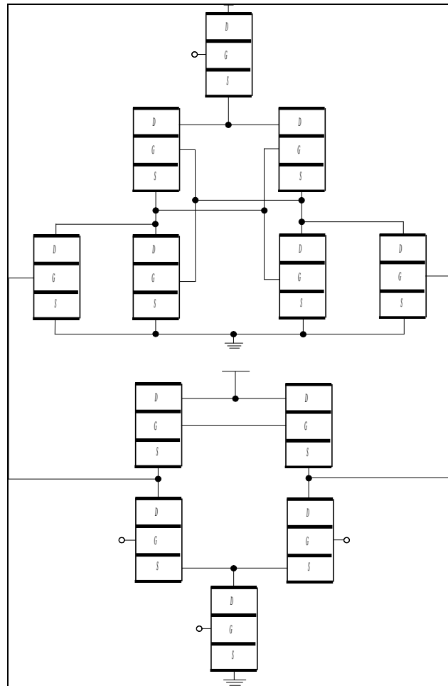
Fig 1: The considered comparator [4]
