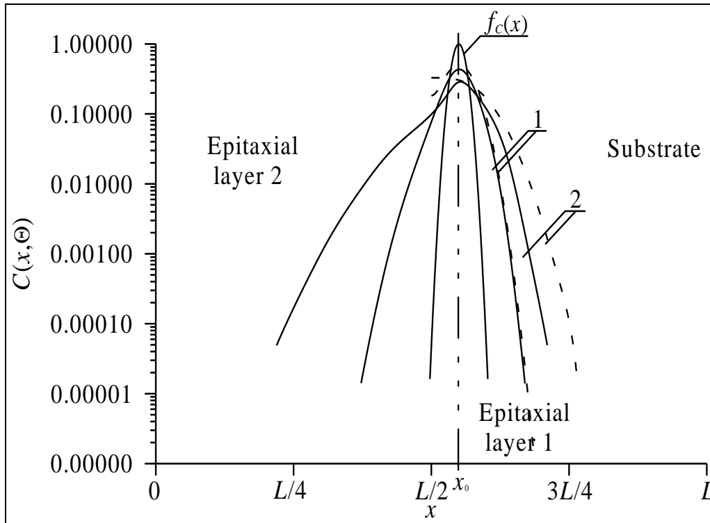
Fig 3b: Calculated distributions of implanted dopant in epitaxial layers of heterostructure. Solid lines are spatial distributions of implanted dopant in system of two epitaxial layers. Dashed lines are spatial distributions of implanted dopant in one epitaxial layer. Annealing time increases with increasing of number of curves
