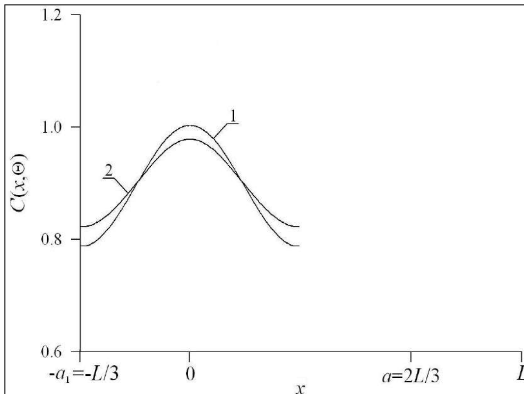
Fig 3a: Distributions of concentration of dopant, infused in average section of epitaxial layer of heterostructure from Figs. 1 in direction parallel to interface between epitaxial layer and substrate of heterostructure. Difference between values of dopant diffusion coefficients increases with increasing of number of curves. Value of dopant diffusion coefficient in this section is smaller, than value of dopant diffusion coefficient in nearest sections
