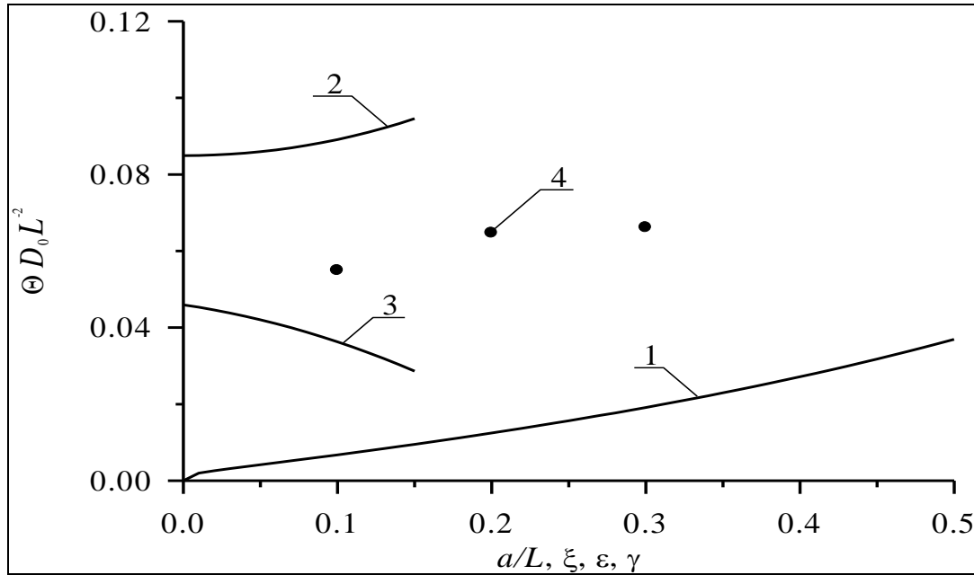
Fig 5b: Dimensionless optimal annealing time of implanted dopant as a function of several parameters. Curve 1 describes the dependence of the annealing time on the relation a/L and \xi = \gamma = 0 for equal to each other values of dopant diffusion coefficient in all parts of heterostructure. Curve 2 describes the dependence of the annealing time on value of parameter \epsilon for a/L=1/2 and \xi = \gamma = 0 . Curve 3 describes the dependence of the annealing time on value of parameter \xi for a/L=1/2 and \epsilon = \gamma = 0 . Curve 4 describes the dependence of the annealing time on value of parameter \gamma for a/L=1/2 and \epsilon = \xi = 0
