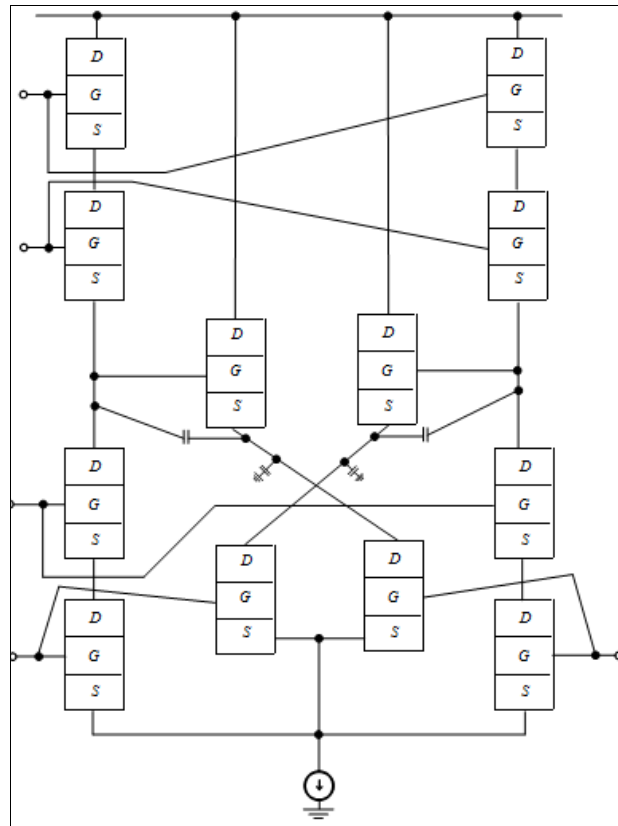
Fig 1a: Structure of the considered amplifier [19]
