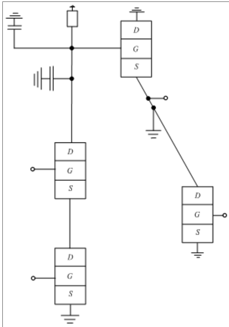
Fig 1a: Structure of the considered amplifier [19]
