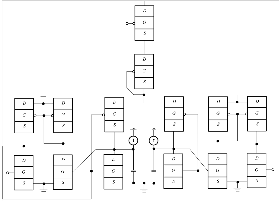
Fig 1a: Structure of the considered oscillator [19]
