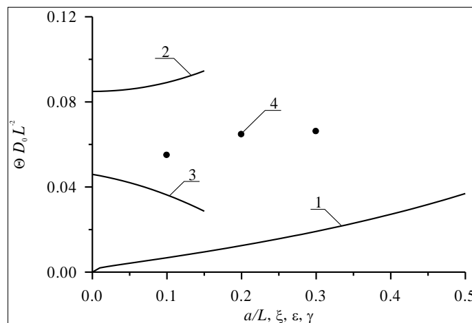
Fig 3b: Dependences of dimensionless optimal annealing time for doping by ion implantation, which have been obtained by minimization of mean-squared error, on several parameters. Curve 1 is the dependence of dimensionless optimal annealing time on the relation a/L and \xi = \gamma = 0 for equal to each other values of dopant diffusion coefficient in all parts of heterostructure. Curve 2 is the dependence of dimensionless optimal annealing time on value of parameter \varepsilon for a/L=1/2 and \xi = \gamma = 0 . Curve 3 is the dependence of dimensionless optimal annealing
