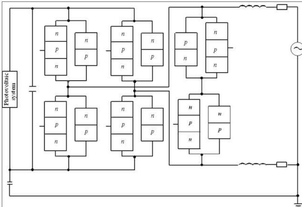
Fig 1a: Structure of the considered inverter. View from top
