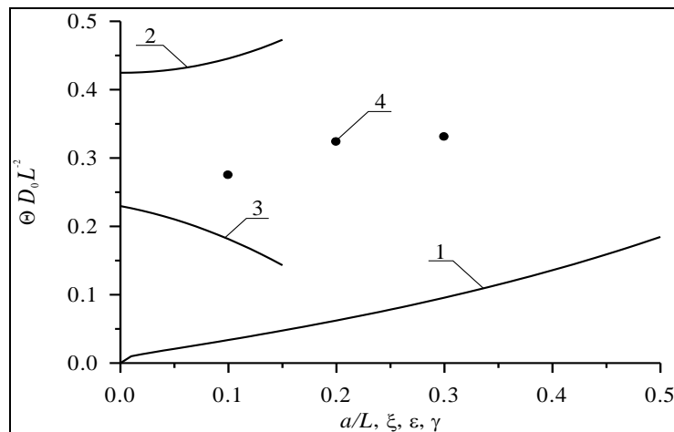
Fig 3a: Dependences of dimensionless optimal annealing time for doping by diffusion, which have been obtained by minimization of mean-squared error, on several parameters. Curve 1 is the dependence of dimensionless optimal annealing time on the relation a/L and \xi = \gamma = 0 for equal to each other values of dopant diffusion coefficient in all parts of heterostructure. Curve 2 is the dependence of dimensionless optimal annealing time on value of parameter \varepsilon for a/L=1/2 and \xi = \gamma = 0 . Curve 3 is the dependence of dimensionless optimal annealing time on value of parameter \xi for a/L=1/2 and \varepsilon = \gamma = 0 . Curve 4 is the dependence of dimensionless optimal annealing time on value of parameter \gamma for a/L=1/2 and \varepsilon = \xi = 0
