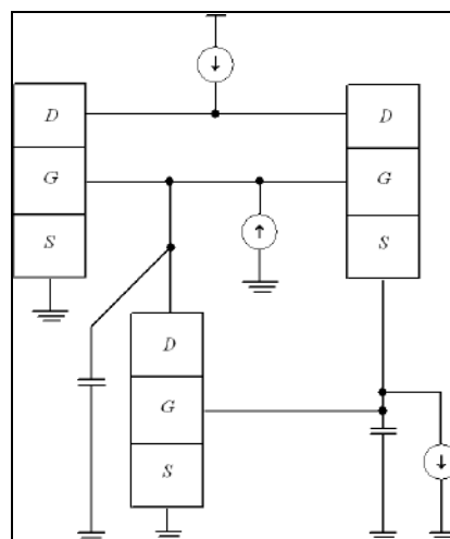
Fig 1a: Structure of the considered filter. View from top
