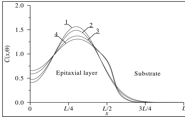
Fig 2b: Distributions of concentration of implanted dopant in heterostructure from Figs. 1 and 2 in direction, which is perpendicular to interface between epitaxial layer substrate. Curves 1 and 3 corresponds to annealing time \Theta = 0.0048(L_x^2 + L_y^2 + L_z^2)/D_0 . Curves 2 and 4 corresponds to annealing time \Theta = 0.0057(L_x^2 + L_y^2 + L_z^2)/D_0 . Curves 1 and 2 corresponds to homogenous sample. Curves 3 and 4 corresponds to heterostructure under condition, when value of dopant diffusion coefficient in epitaxial layer is larger, than value of dopant diffusion coefficient in substrate
