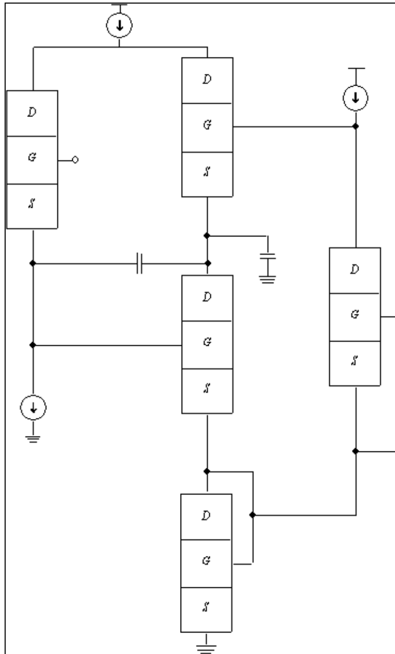
Fig 1a: Structure of the considered filter [19]
