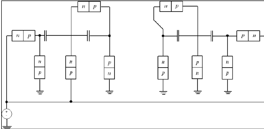
Fig 1a: Structure of the considered symmetrical multiplier [19].
